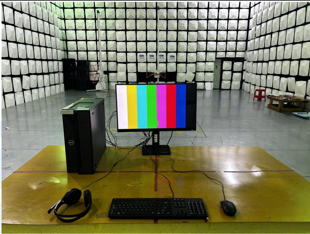
Radiated emission Test Setup (30MHz~1GHz)_ 10 Meter test distance
